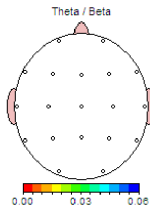
Figure 3. Spectral brain-maps: FFT Power Ratio Group t-test (p-Values)
